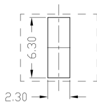
PCB LAYOUT
