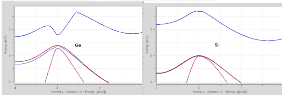
Band structure plot for Si, Ge.
