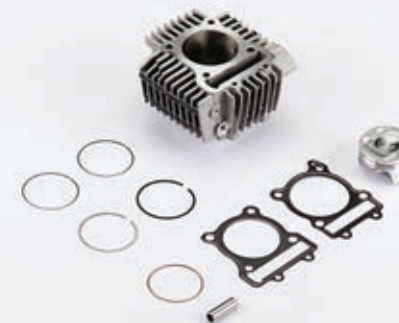
KIT 212cc 212cc KIT
