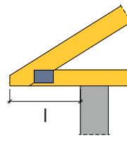
Kragarm
