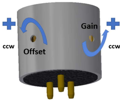
Figure 15. Adjustment the Wheatstone bridge offset (zero point of calibration straight line) and amplifier gain (slope of calibration straight line). If necessary, trimmer settings can be altered by means of a screw driver. Note, that both holes have a diameter of 1.8 mm. A ceramic type instrument (e.g., CD-15) is
