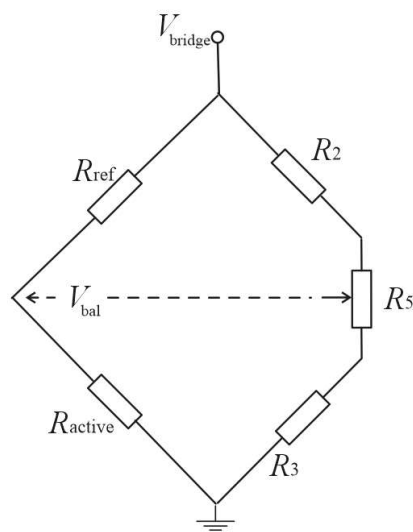
Figure 16. Wheatstone bridge with active and reference sensor element (schematic).
