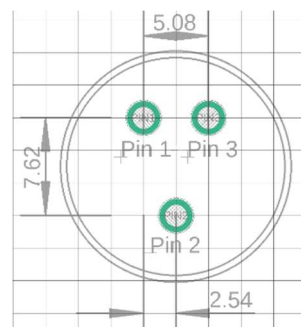
Figure 17: Footprint (dimensions shown in millimeter)
