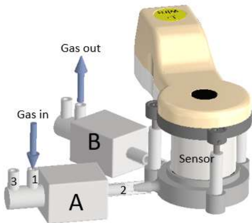
Figure 13. Special setup to determine the response and decay time of the sensor. Here, the evaluation kit PGA-ADC 3.3 is used to apply the 12 V voltage and to determine the signal voltage V_{\text{SIGNAL}} of the sensor. A flow of 2 vol-% H_2 in air with 50 sccm/min flows into the system at the “gas in” through port 1 of valve A. The valve can be switched electrically to pass the flow through port 3 to the ambient air or port 2 to the sensor, attached to a small test chamber. Valve B is operated together with valve A and cut off the test chamber from the outlet if A is switched into the 1-3 position.
