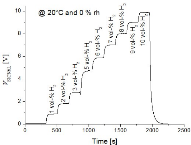
Figure 12. Sensor signal of H2-CNI 0V-I WR as a function of time for hydrogen volume fractions from 1 to 10 vol-% in air at a total flow of 50 sccm/min. Note that unlike the 0V and 0V ULTD sensors, this wide range WR type provides an output signal from 0 to 10 V.
