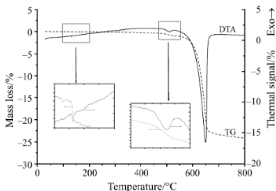
Figure 1. TG and DTA curve recorded at 5°C min -1 of FeS 2
